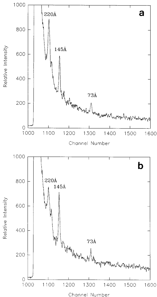
FIGURE 5 Meridional profiles of a MgATP-relaxed bundle (a) and the same bundle relaxed in MgAMP-PNP (b). Thick filament related meridional reflections at 220, 145, and 73 Å are indicated.
