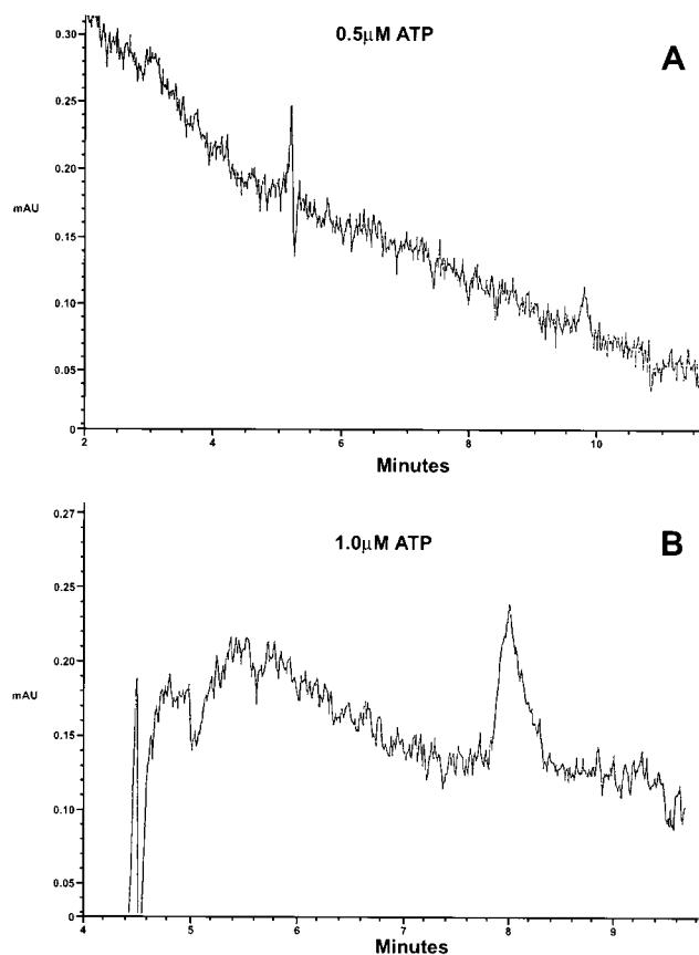
FIGURE 9 HPLC traces of 0.5 \mu M (A) and 1 \mu M (B) ATP used to determine the limit of detectability of this nucleotide. All samples were run under the same conditions as in Fig. 8.
