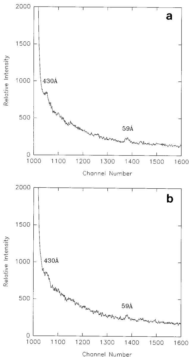
FIGURE 4 Profiles of off-meridional vertical slices through the two-dimensional x-ray diffraction patterns shown in Fig. 3. (a) 10 mM MgATP. (b) 25 mM MgAMP-PNP. Myosin layer line at 430 Å and actin layer line at 59 Å are indicated.
