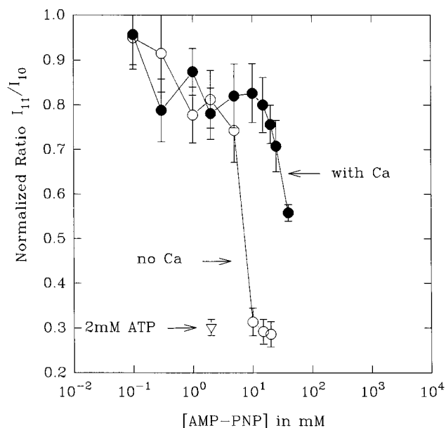
FIGURE 1 The equatorial intensity ratio I_{11}/I_{10} used as a measure of the fraction of cross-bridges attached to actin as a function of increasing MgAMP-PNP concentration. Single rabbit psoas muscle fibers were studied in CaEGTA (●), in EGTA solution (○), and in 2mM MgATP with no AMP-PNP (▽). Temperature, 1°C. Ionic strength, 170 mM. Sarcomere length, 2.3–2.4 \mu\text{m} . The rigor data point in EGTA solution was set to 1.0 (the actual ratio was \sim 3.0 ). Other data points were normalized to this value.
